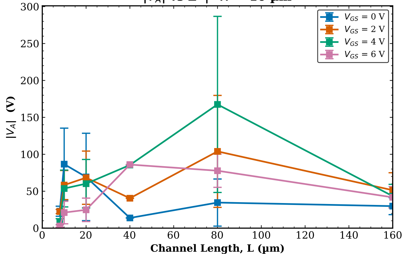
TFT3 Combined (Tr. 1 & 2) |V_A| vs L | W = 10\text{ }\mu\text{m}
